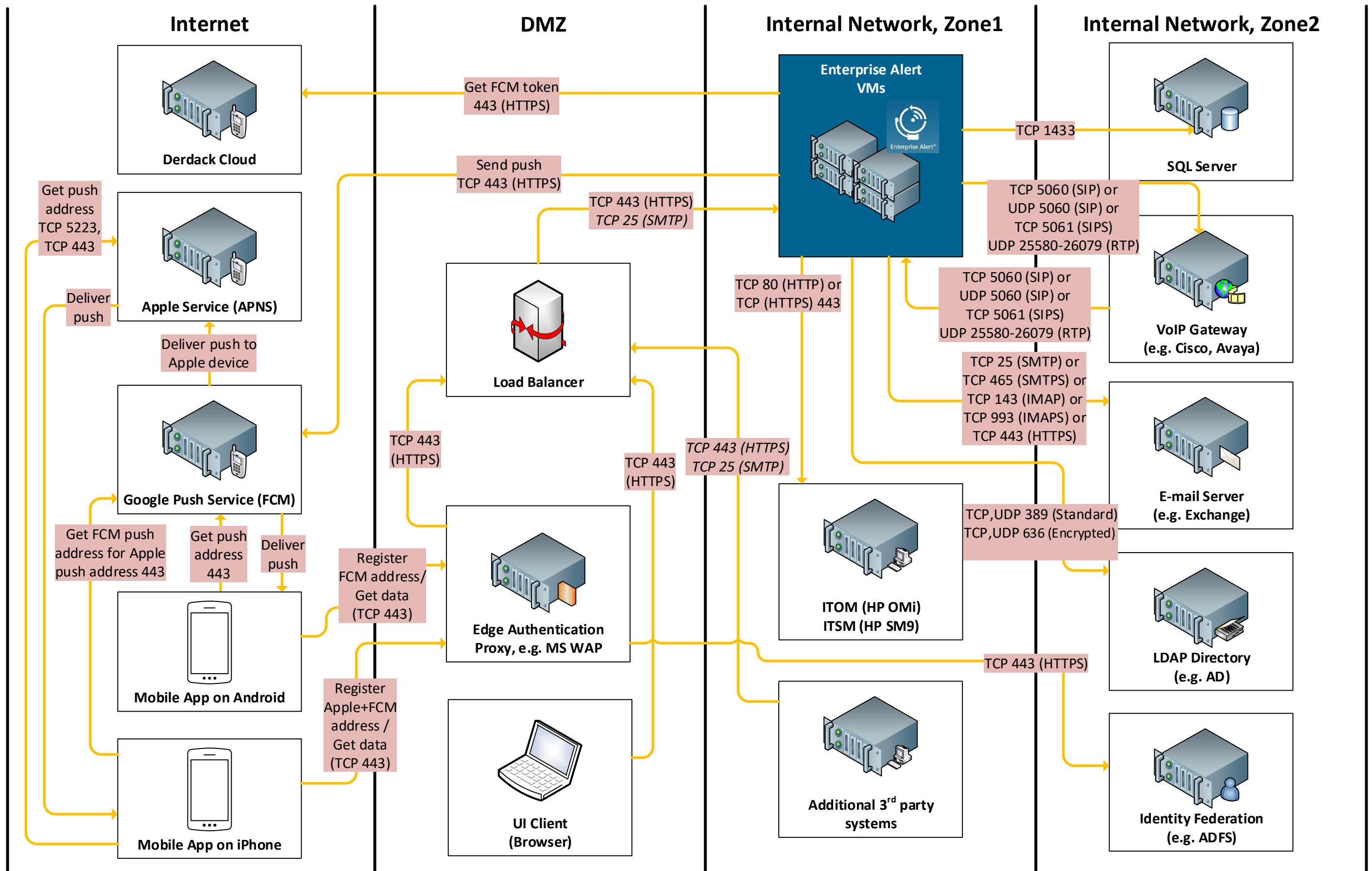
Derdack Enterprise Alert – Typical Network Deployment Topology. 2020-05-29
